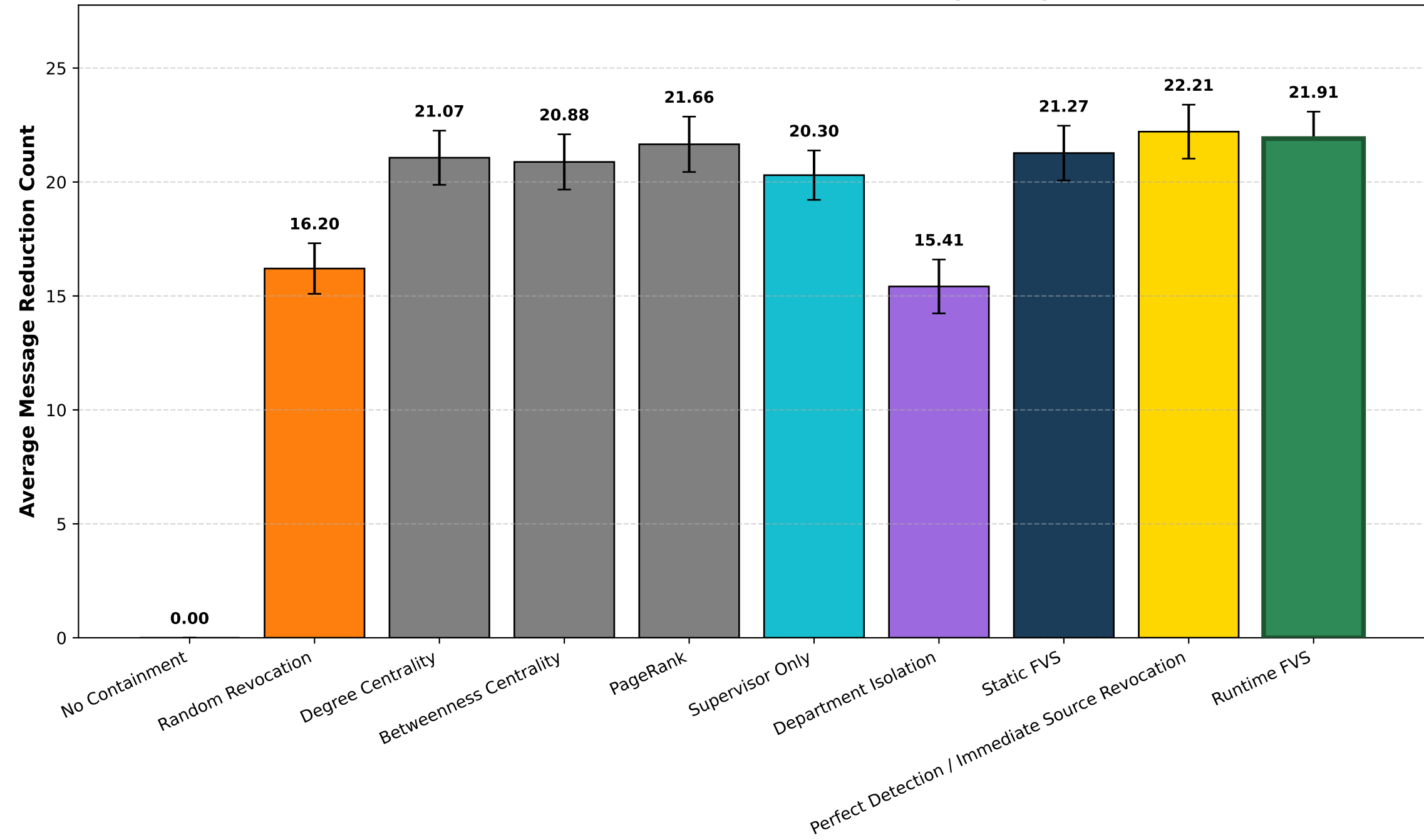
Communication Overhead Reduction by Policy
